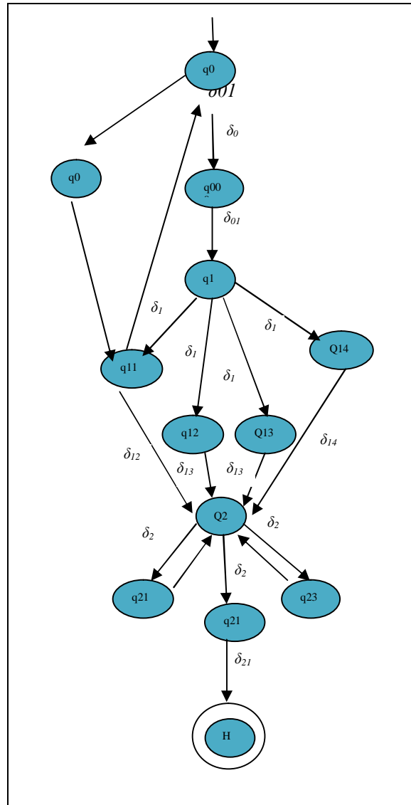
Fig 2: Constructed Finite State Machine
