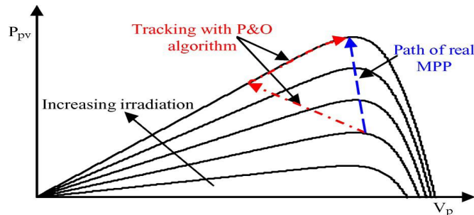
Fig. 6. Deviation from the MPP with the P&O algorithm under rapidly changing irradiance.
