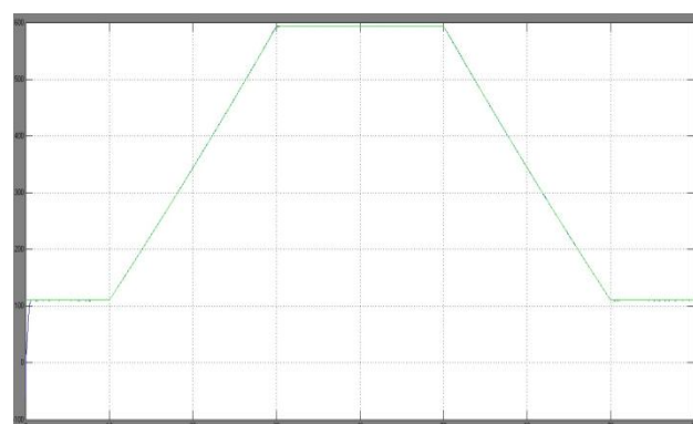
Fig. 14. PV system voltage with the voltage during a trapezoidal irradiation profile. MPP voltage during a trapezoidal irradiation
