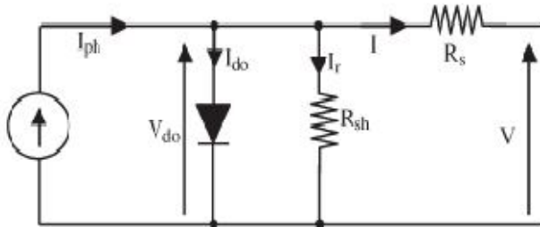
Fig. 2. Solar cell electrically equivalent circuit.
