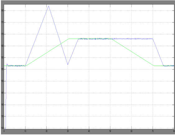
Fig.13 PV array voltage with classical P&O and theoretical MPP modified MPPT and theoretical
