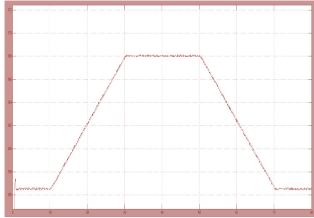
Fig. 14. PV system voltage with the voltage during a trapezoidal irradiation profile. MPP voltage during a trapezoidal irradiation
