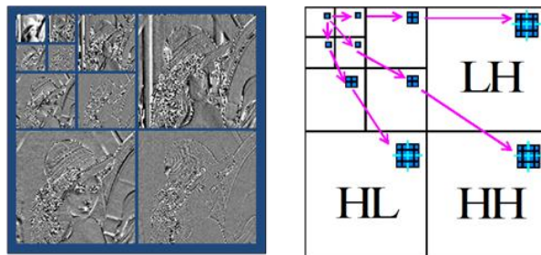
Fig. 3 Wavelet Decomposition
