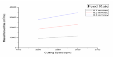
Figure 5.7 Depth of Cut as 0.5 mm
