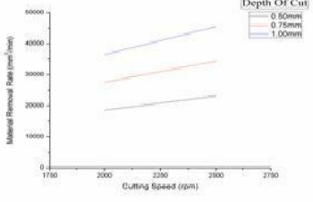
Figure 5.5 Feed Rate as 0.2 mm/rev
