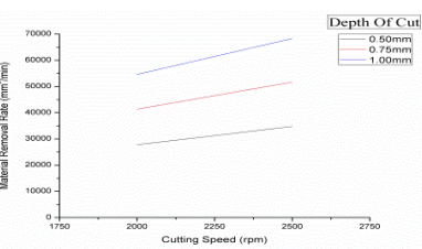
Figure 5.6 Feed Rate as 0.3 mm/rev
