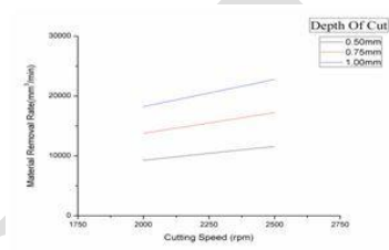
Figure 5.4 Feed Rate as 0.1mm/rev
