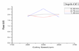
Figure 5.19 Feed Rate as 0.2 mm/rev
