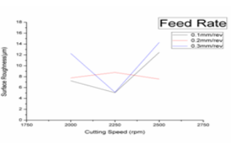
Figure 5.18 Depth of Cut as 0.75 mm
