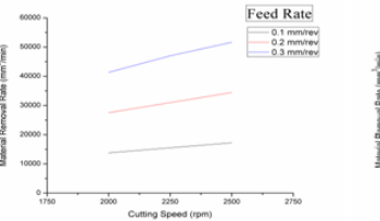
Figure 5.8 Depth of Cut as 0.75 mm
