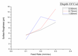
Figure 5.10 Cutting Speed as 2000 rpm
