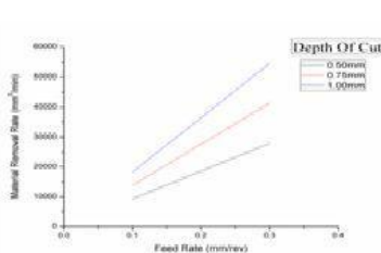
Figure 5.1 Cutting Speed as 2000 rpm
