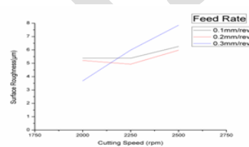
Figure 5.17 Depth of Cut as 0.5 mm
