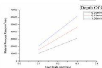
Figure 5.2 Cutting Speed as 2250 rpm
