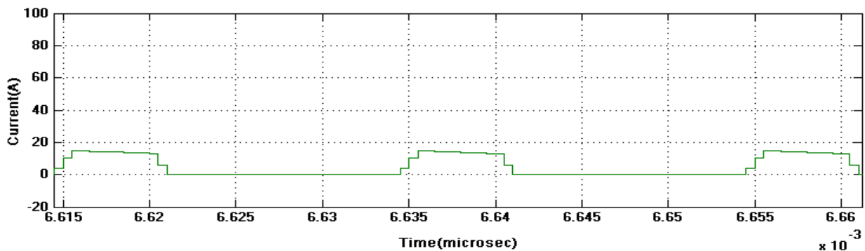
Figure.22. Output current waveform for proposed converter in CCM operation at I_{d0} .
