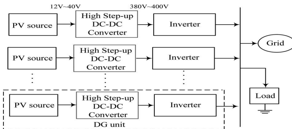
Figure.1.1. PV Distributed System
