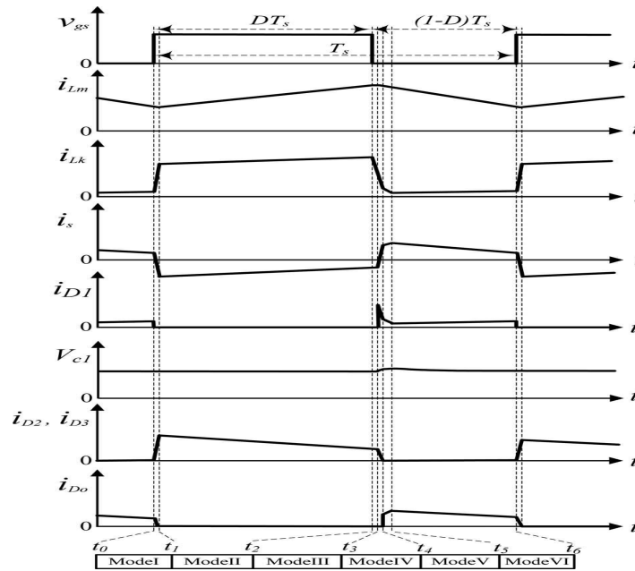
Figure.8. Some typical key waveforms of the proposed converter at CCM operation.
