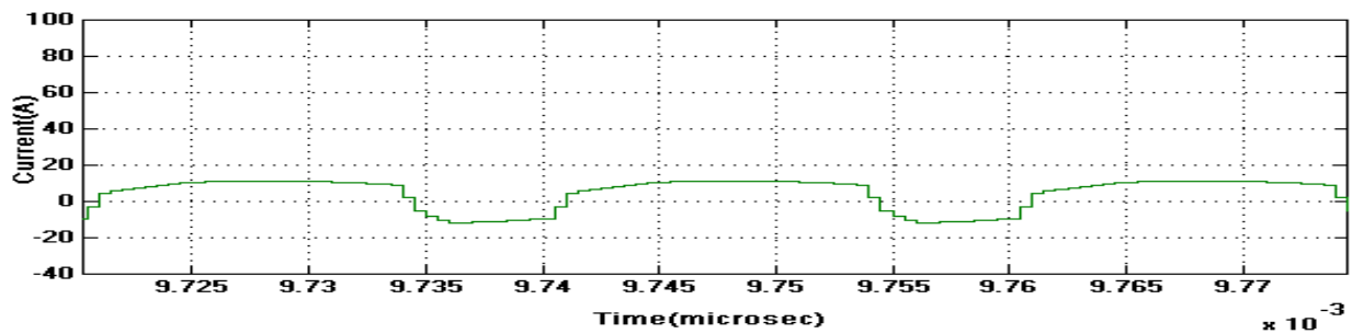
Figure.17 Output current waveform for proposed converter in CCM operation at I_S .
