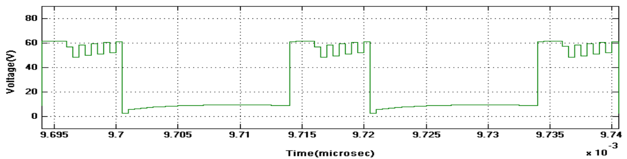
Figure.18. Output voltage waveform for proposed converter in CCM operation at V_{ds} .
