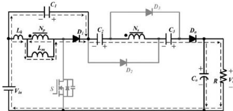
Figure.7. Current flowing path of proposed converter CCM Mode VI operation
