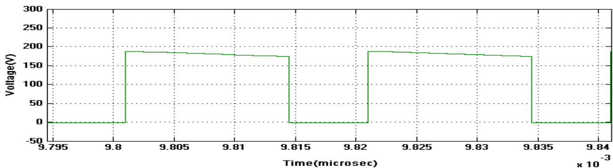
Figure.23. Output voltage waveforms for proposed converter in CCM operation at V_{d0} .
