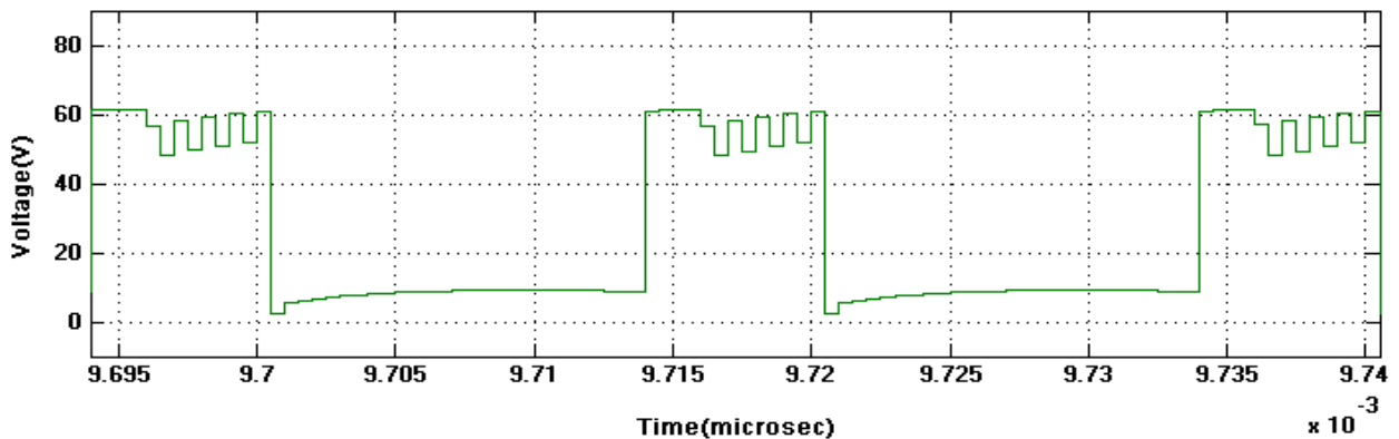
Figure.15. Output voltage waveform for proposed converter in CCM operation at V_{ds} .
