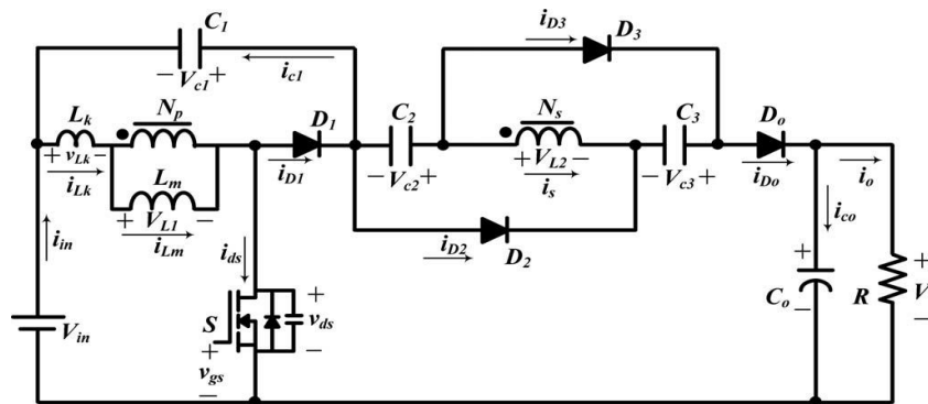
Figure.1. Circuit Configuration of the proposed converter
