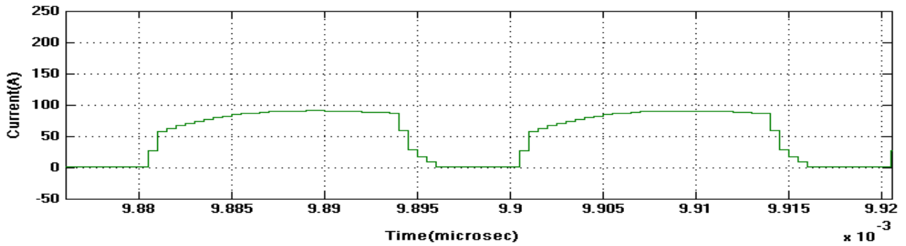
Figure.16. Output current waveform for proposed converter in CCM operation at I_{lk} .
