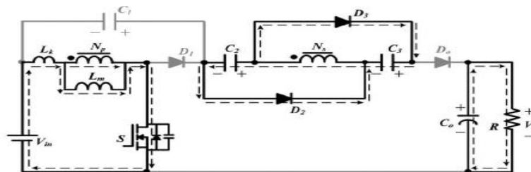
Figure.3. Current flowing path of proposed converter CCM Mode II operation.
