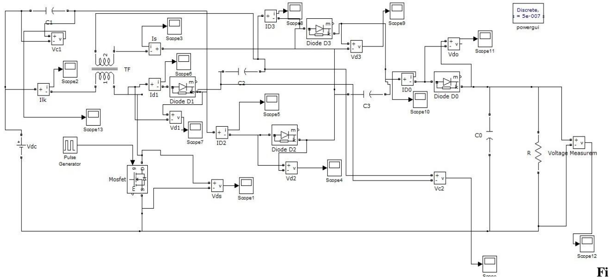
Figure.13 MATLAB/Simulink Model of the Proposed Converter under Full-Load condition P_o=400W .
