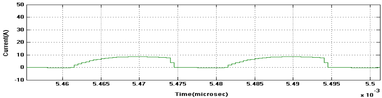
Figure.20 Output current waveform for proposed converter in CCM operation at I_{d3} .
