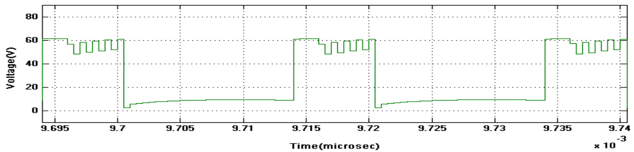
Figure.21. Output voltage waveform for proposed converter in CCM operation at V_{ds} .
