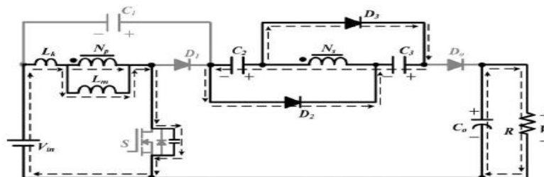
Figure.4. Current flowing path of proposed converter CCM Mode III operation.
