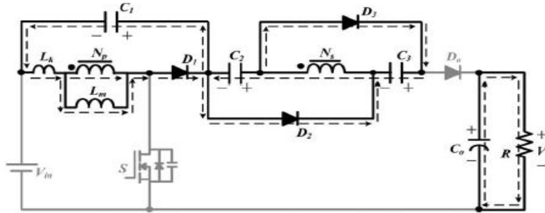
Figure.5. Current flowing path of proposed converter CCM Mode IV operation
