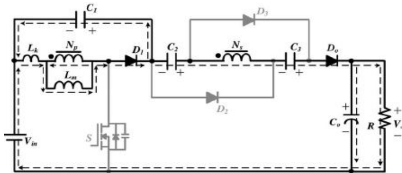
Figure.6. Current flowing path of proposed converter CCM Mode V operation
