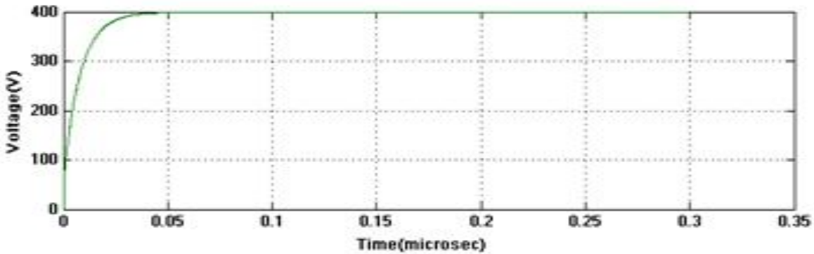
Figure.14. Output voltage waveform for proposed converter in CCM operation
