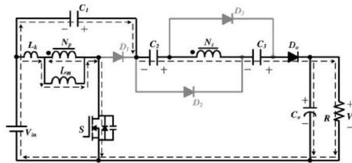
Figure.2. Current flowing path of proposed converter CCM Mode I operation.
