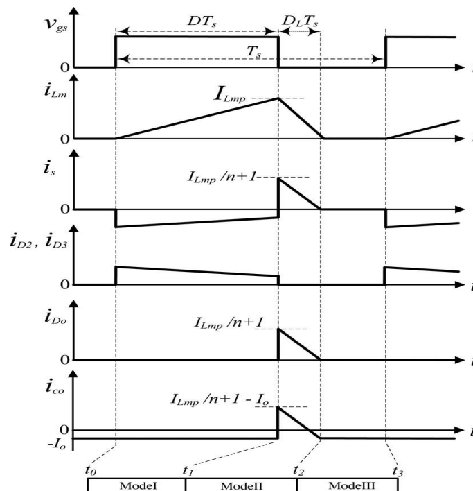
Figure.12. Some typical key waveforms of the proposed converter at DCM operation.
