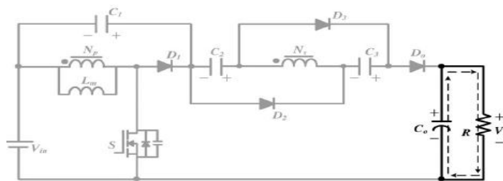
Figure.11. Current flowing path of proposed converter DCM Mode III operation
