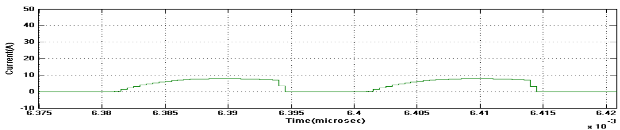
Figure.19 Output current waveform for proposed converter in CCM operation at I_{d2} .
