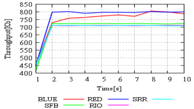
Figure 5: Throughput of bottleneck link (3–4) for Pareto Traffic
