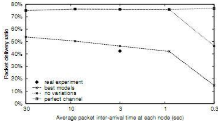
Fig.2. Packet delivery ratio with USVGM protocol
