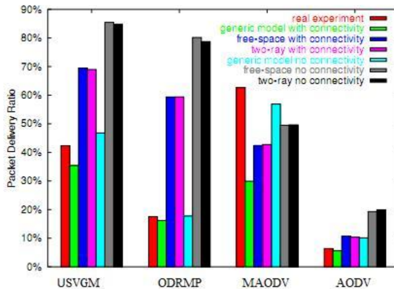
Fig.3. Simulation results of various protocol packet delivery ratio.
